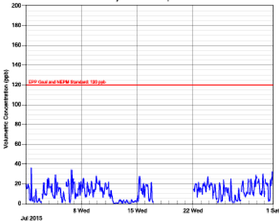
NO 2 , 1 hour average Royal Brisbane Hospital
