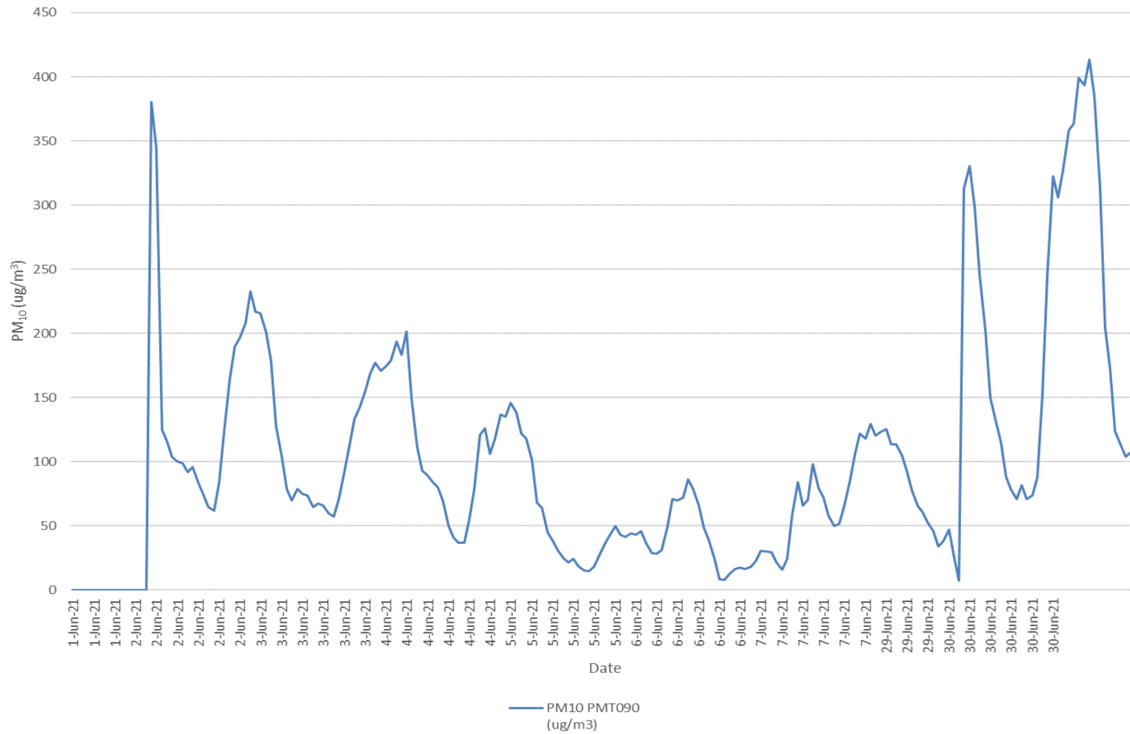
Figure 4: In-stack monitoring, PM 10 results for June 2021 (60min time-weighted average)
