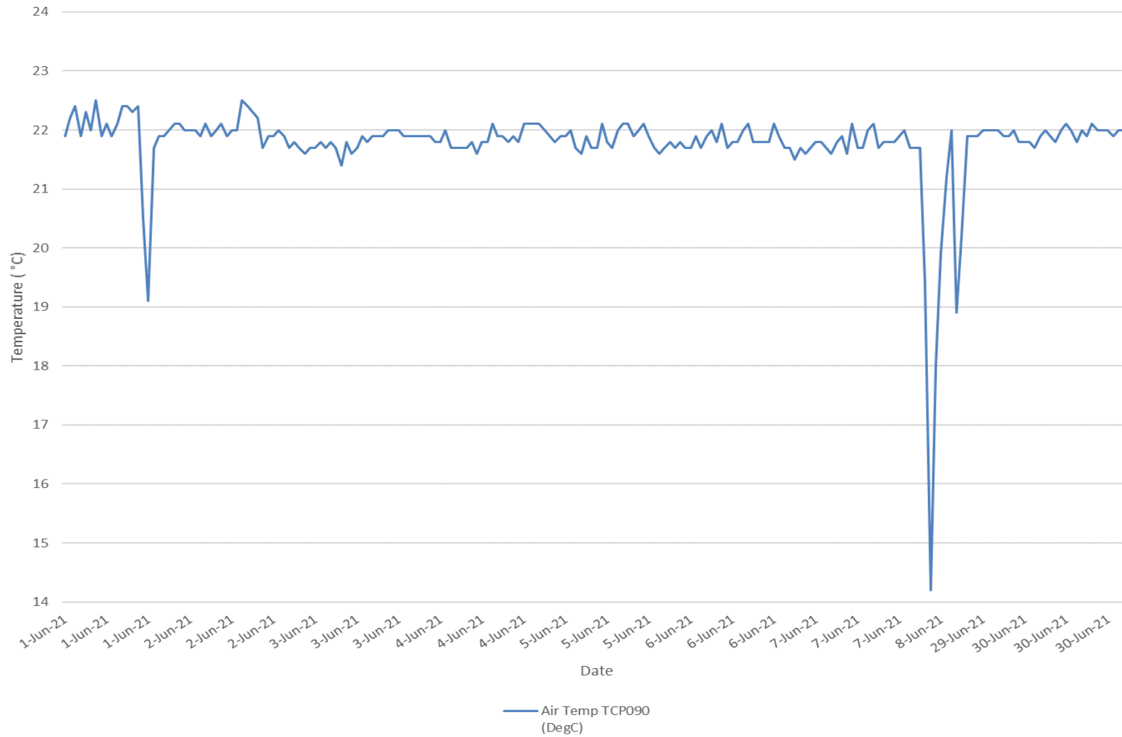
Figure 6: In-stack monitoring, temperature results for June 2021 (60min time-weighted average)
