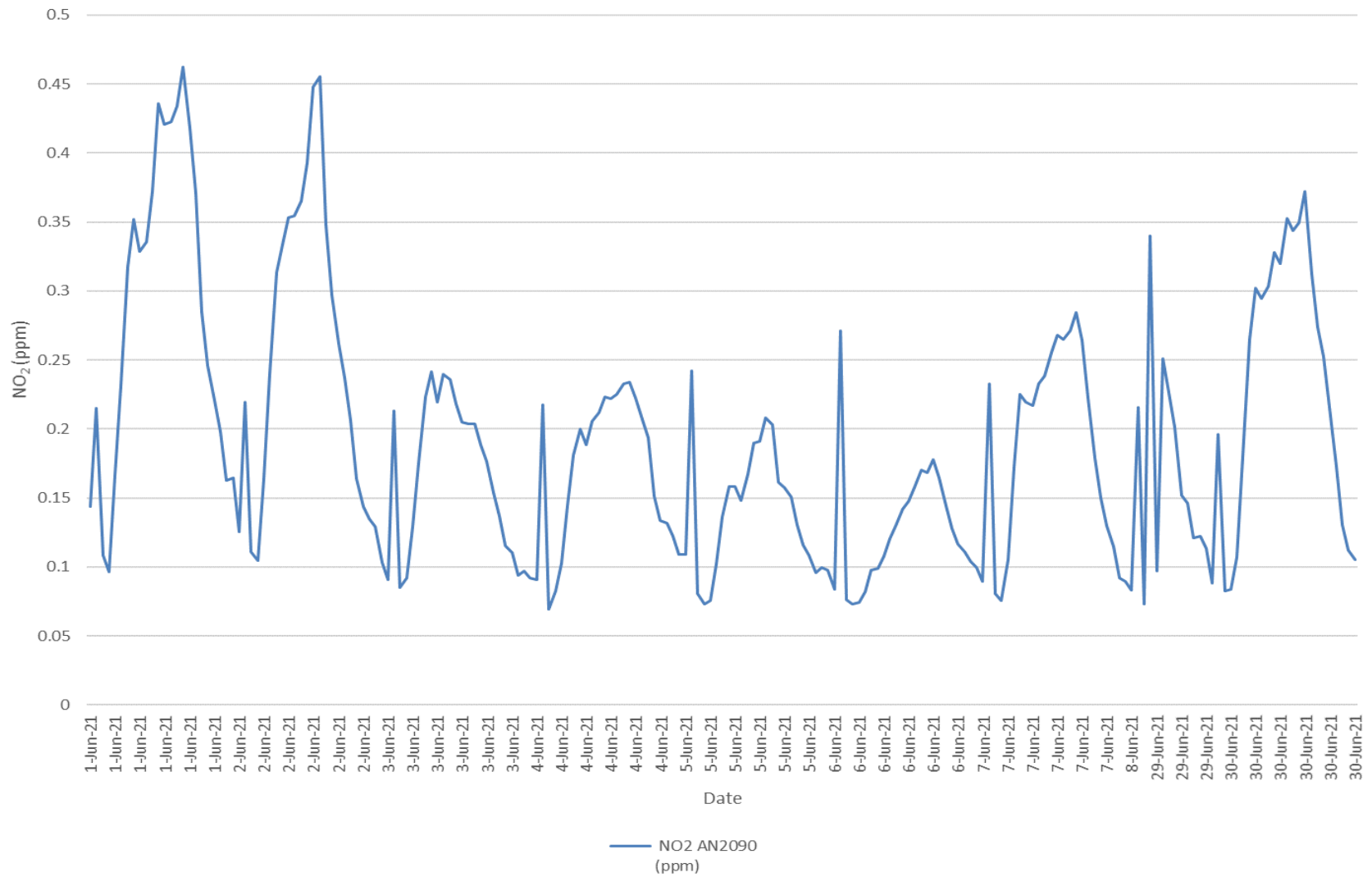
Figure 2: In-stack monitoring, NO 2 results for June 2021 (60min time-weighted average)
