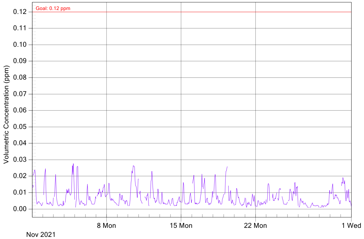
Figure 3: M4 East Haberfield Public School Station - NO 2 1-Hour Averages Graph for November 2021
