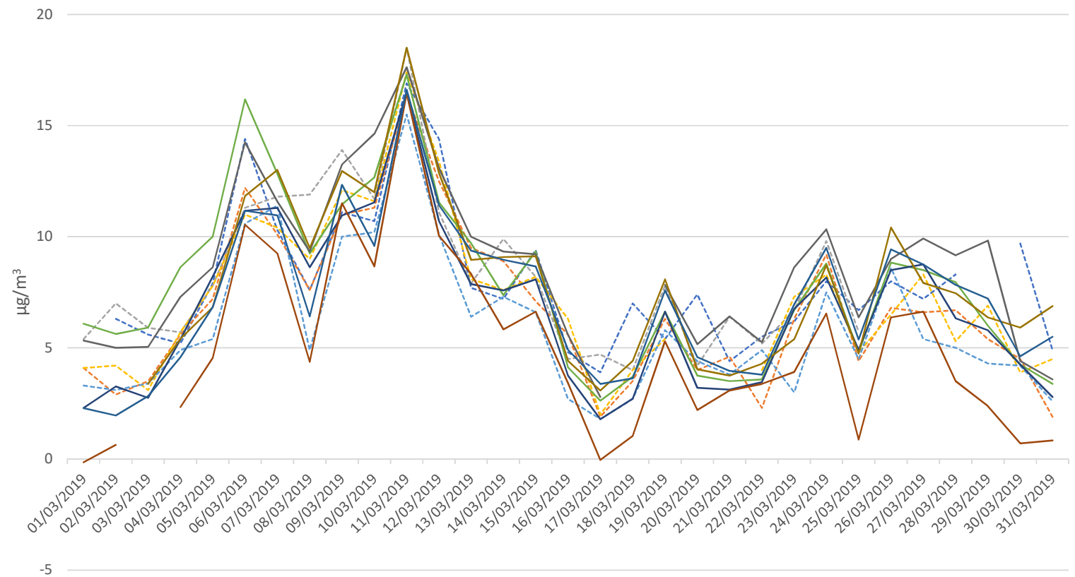
Comparison of WestConnex M4 sites with EPA Sites PM 2.5 24hr average March 2019
