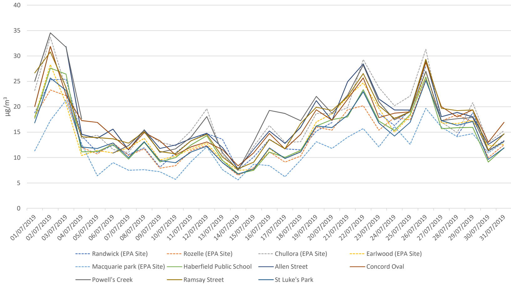
Comparison of WestConnex M4 sites with EPA Sites PM 10 24hr average July 2019
