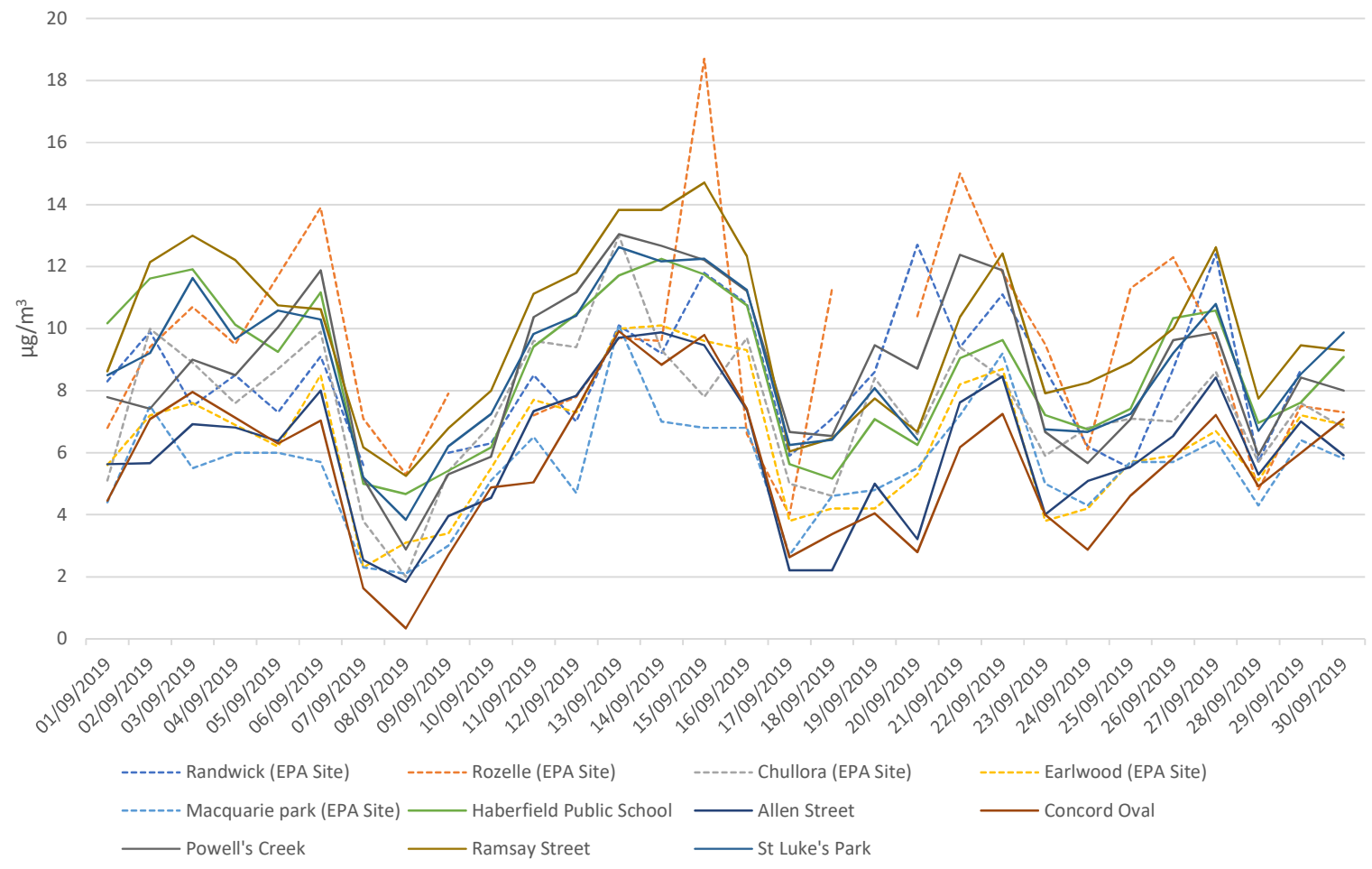
Comparison of WestConnex M4 sites with EPA Sites PM 2.5 24hr average September 2019
